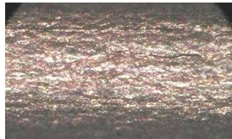
Temper:SH, Thickness: 0.1mm(TS=1.05GPa) Temper:SH, Thickness: 0.08mm(TS=1.03GPa) Fig.1 Surface appearance of 90° W shaped bending test specimens NKT322
