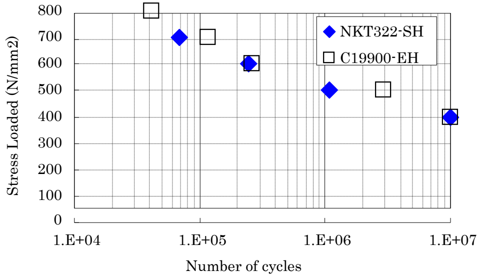
Fig. 2 Comparison of Fatigue Strength
